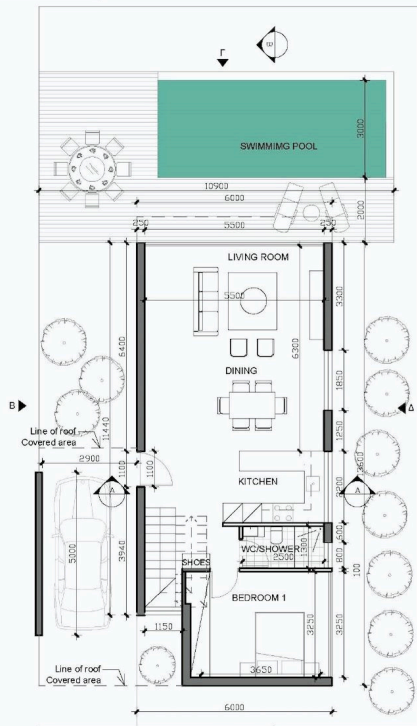
1st Floor = 78.5 sq.m GROUND FLOOR PLAN 72 SQM
