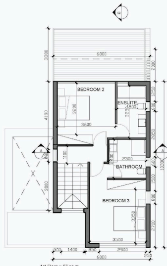
1st Floor = 57 sq.m FIRST FLOOR PLAN 60 SQM
