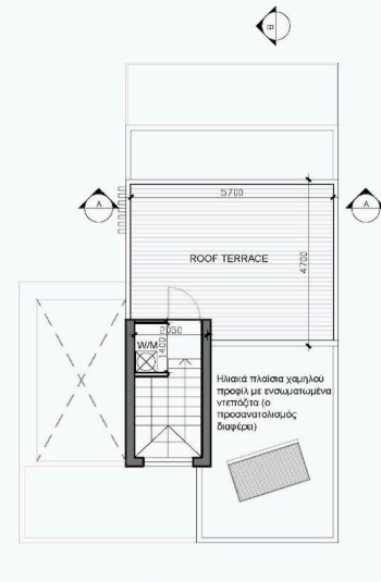
1st Floor = 10 sq.m ROOF PLAN 10 SQM TOTAL AREA 142 SQM
