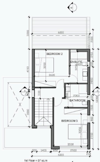
FIRST FLOOR PLAN 60 SQM
