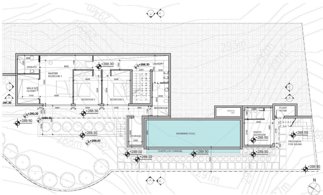
BASEMENT PLAN SCALE 1:100
