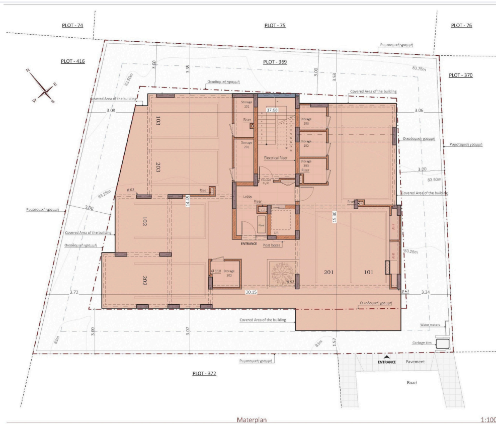
Masterplan
