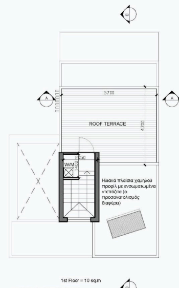
ROOF PLAN 10 SQM TOTAL AREA 142 SQM
