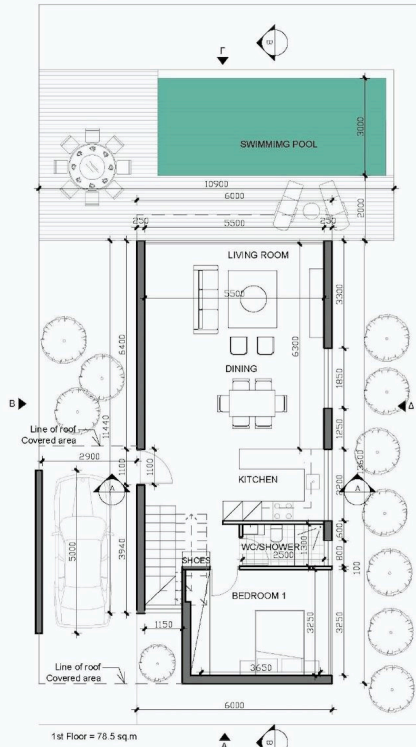
GROUND FLOOR PLAN 72 SQM
