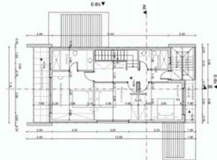
Type B - First Floor
